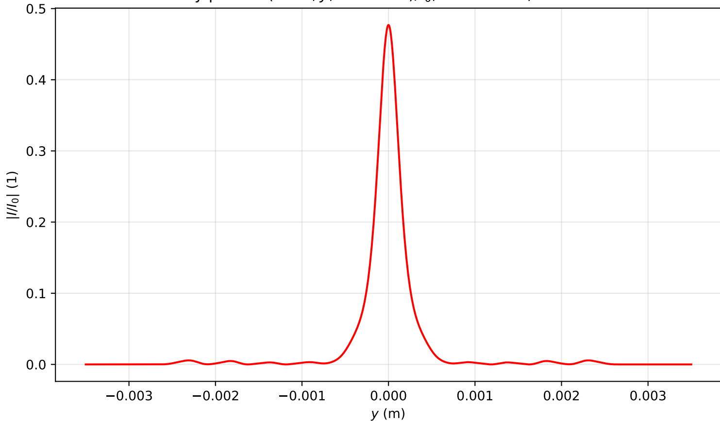
Intensity profile I(x=0, y, z=3.184)/I_0 , \text{Pin}=7.0\text{Pcr} , artificial time
